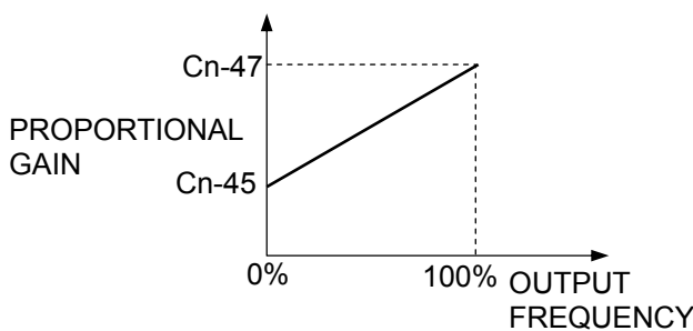
Fig. 15 Relation between Output Frequency and Proportional Gain
