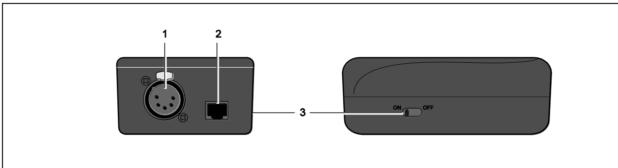
Fig. 14: Micro R-512 Lite, side view
