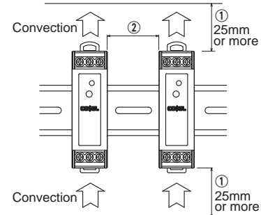
Fig.5.3 Installation clearance
