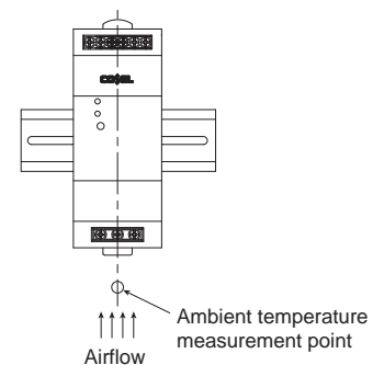
Fig.5.19 Ambient temperature measurement point
