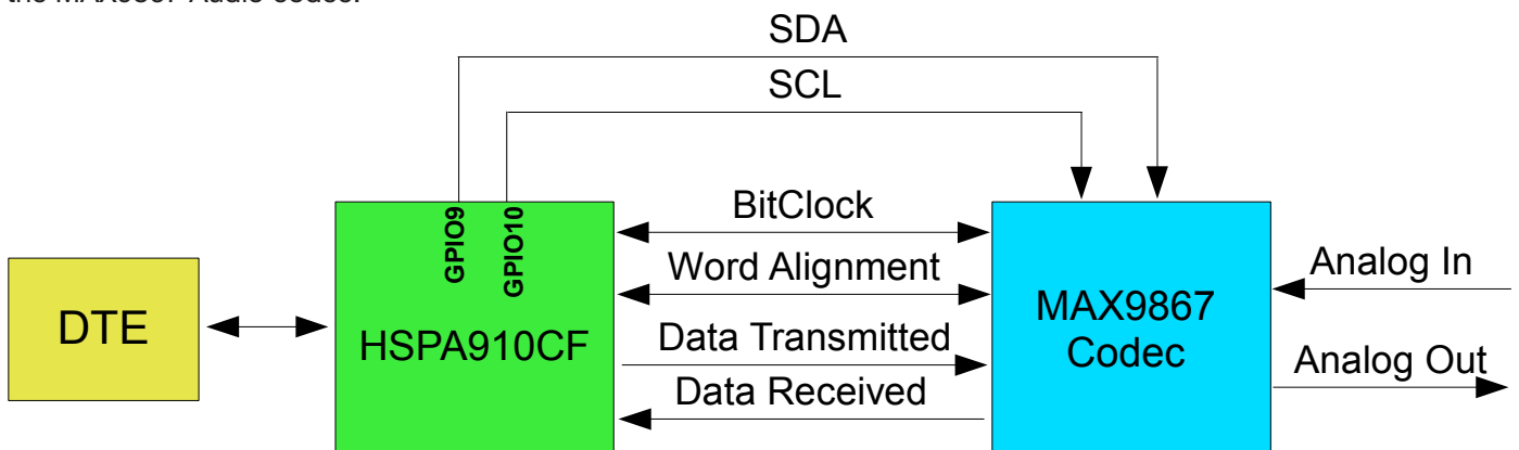
Figure 9 DVI Block Diagram
