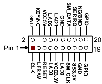
TPM Header
