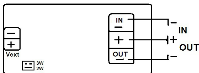
Two wire system wiring diagram
