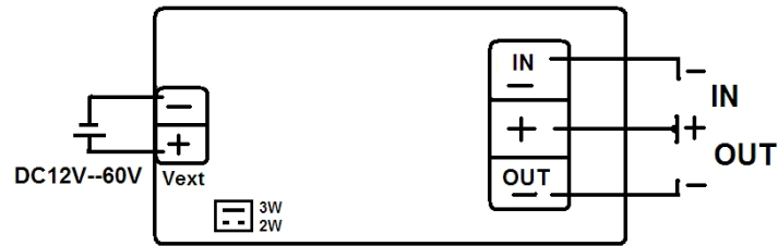
Three wire system wiring diagram
