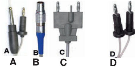
GIMA HF122 Storz Valleylab (autobipolar) 4mm Banana Plugs Valley Lab Eschman Arthrex OPES
