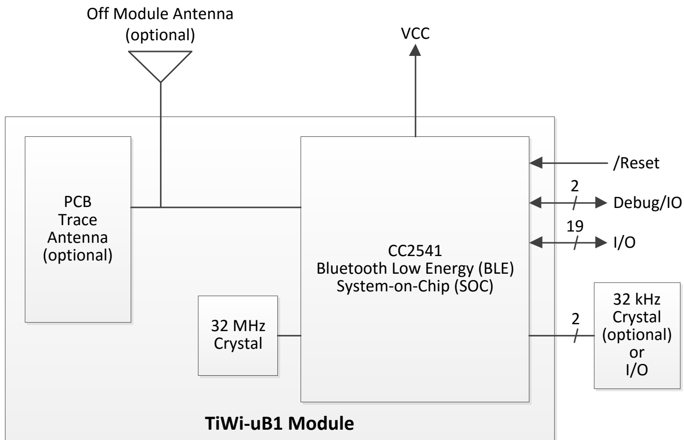
Figure 1 TiWi-uB1 Module Block Diagram
