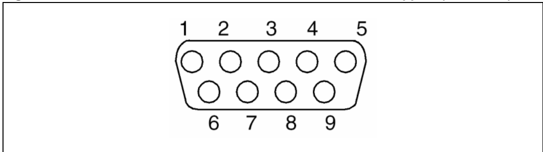
Figure 10. RS232 connector CN5 with RTS/CTS handshake support (front view)
