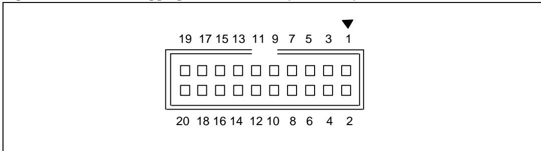
Figure 12. JTAG debugging connector CN7 (front view)
