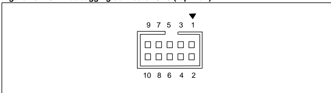
Figure 13. SWD debugging connector CN9 (top view)
