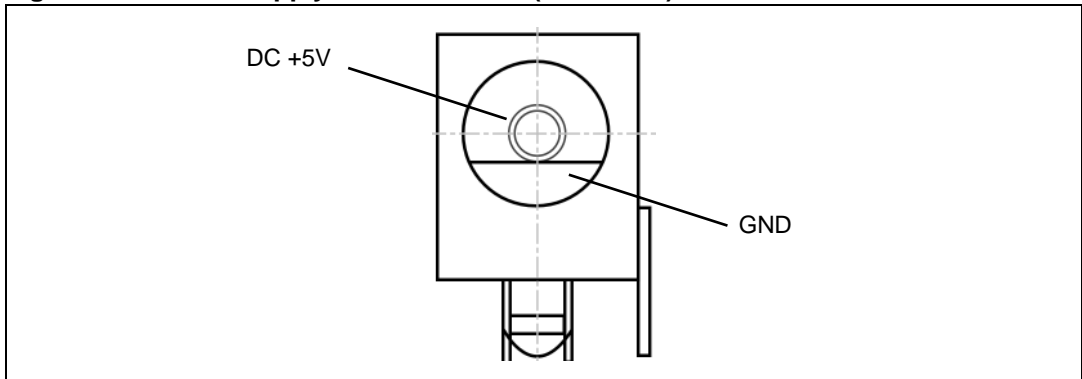
Figure 9. Power supply connector CN4 (front view)
