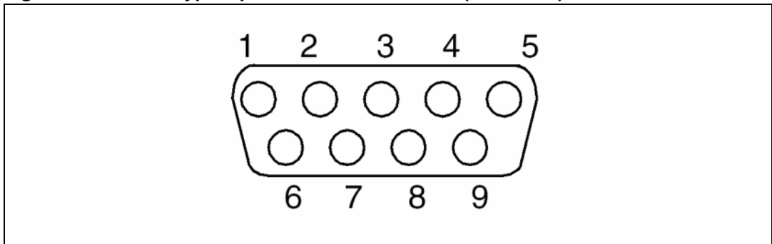
Figure 7. CAN D-type 9-pin male connector CN2 (front view)
