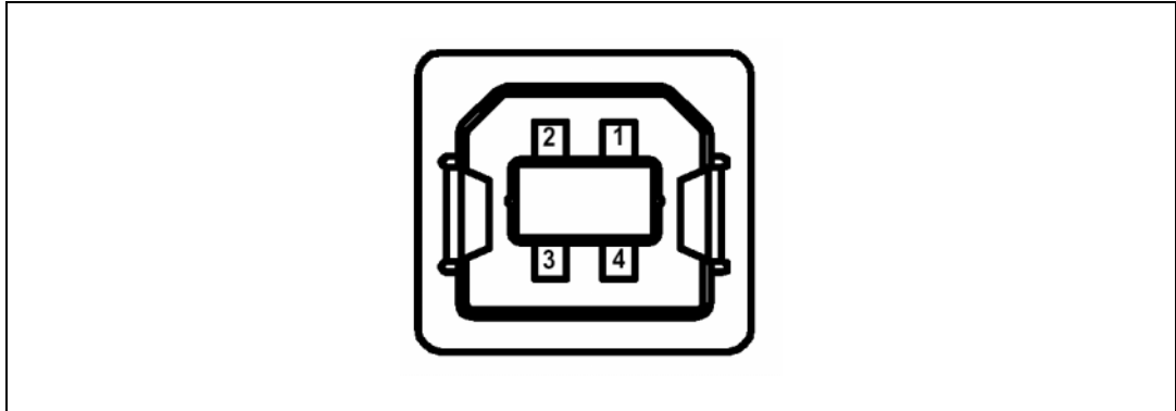
Figure 6. USB type B connector CN1 (front view)
