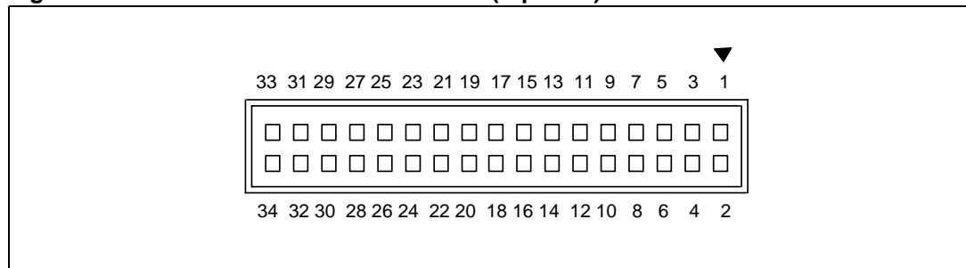
Figure 15. Motor control connector CN14 (top view)
