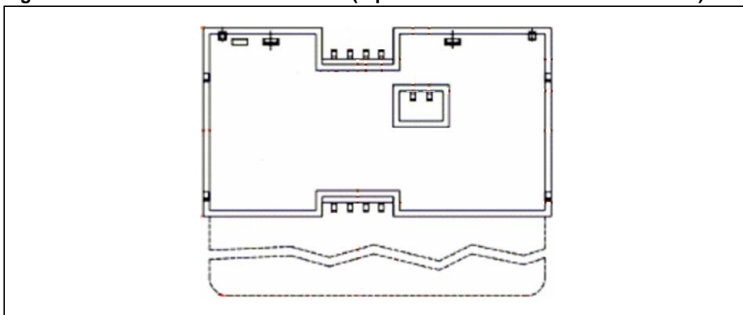
Figure 17. Smartcard connector CN16 (top view of connector underneath PCB)
