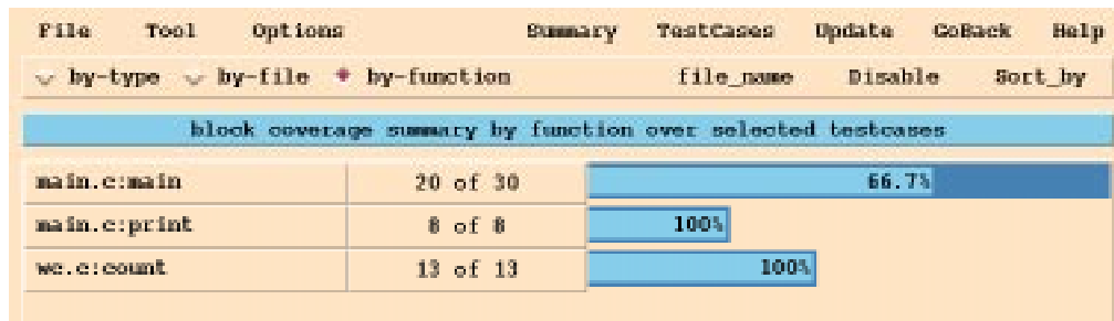
Figure 2-10 The coverage summary by-function , after executing wordcount.2
