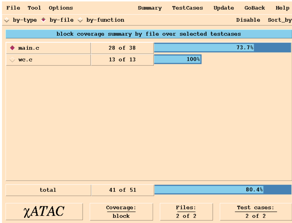
Figure 2-8 The coverage summary by-file after executing wordcount.2
