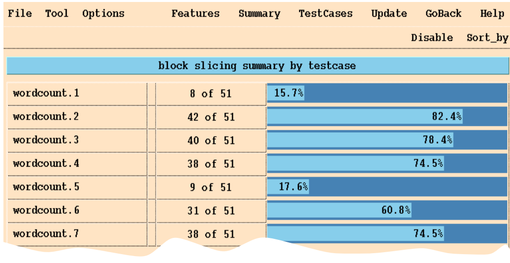
Figure 12-6 The updated coverage summary by test case
