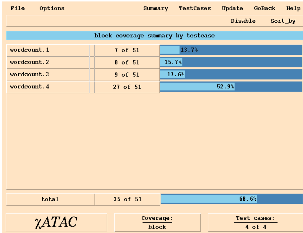
Figure 9-5 A test case display
