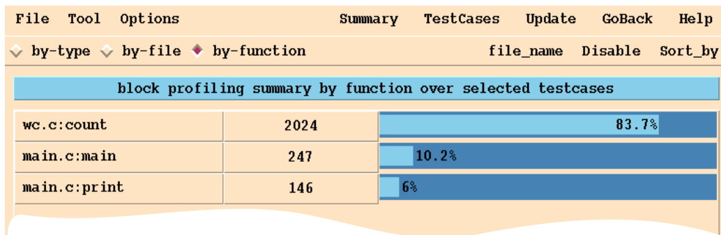
Figure 14-2 A block profiling summary by-function over all selected test cases
