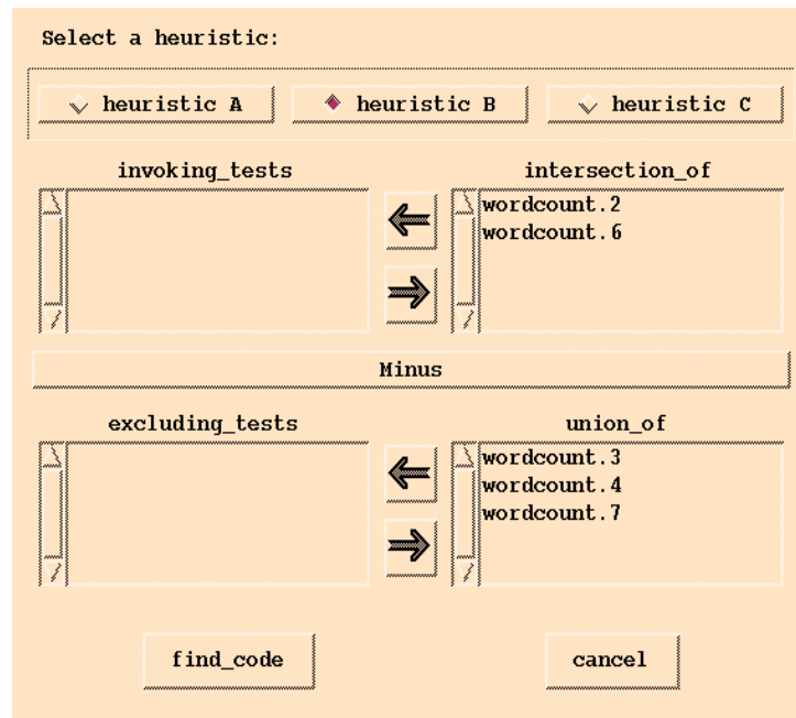
Figure 12-14 Heuristics window with heuristic B selected
