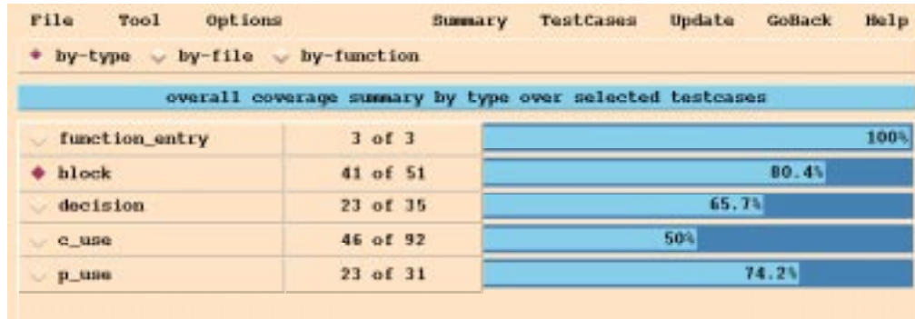
Figure 2-9 The coverage summary by-type after executing wordcount.2
