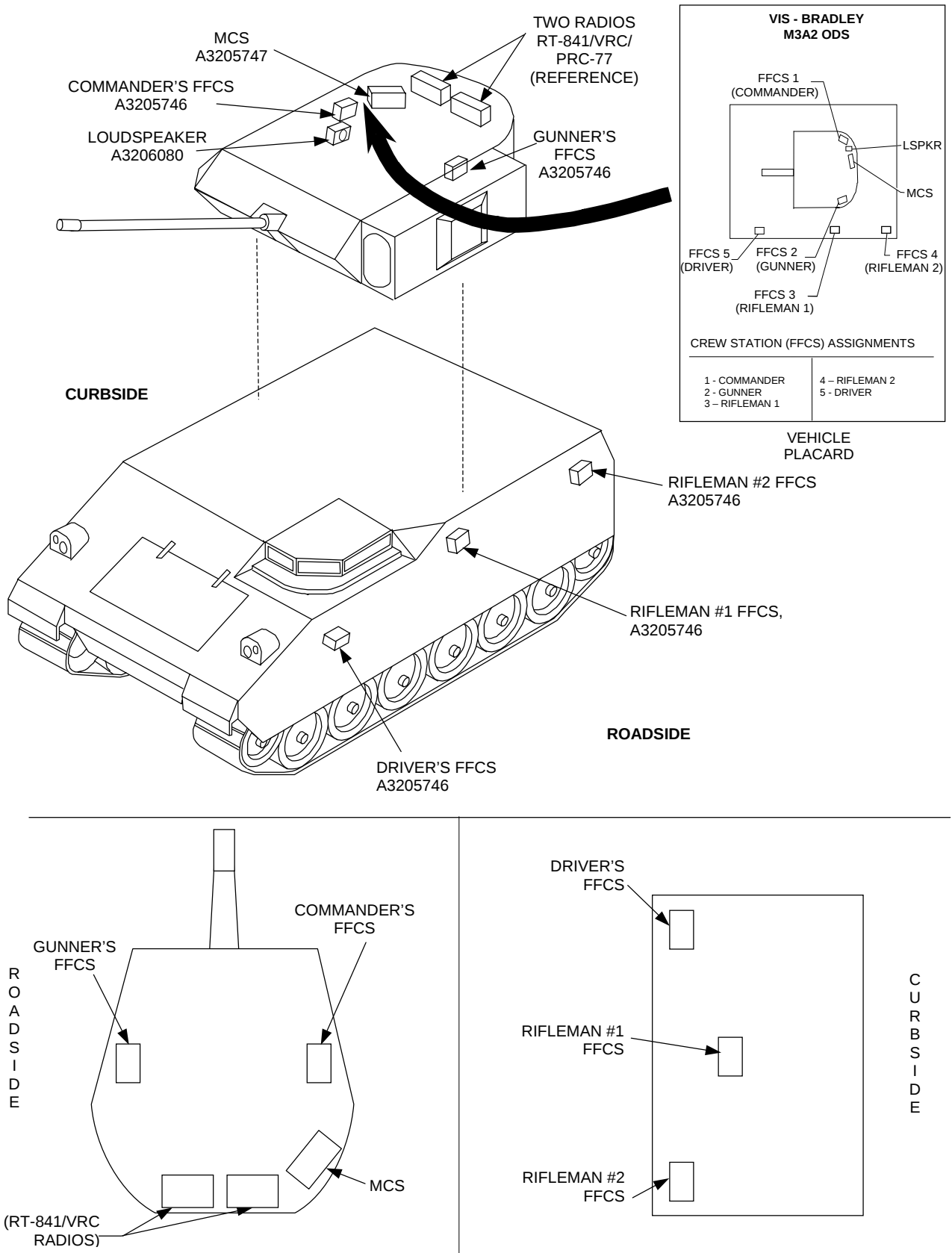
Figure 2-19. M3A2 ODS Bradley Equipment Location Diagram
