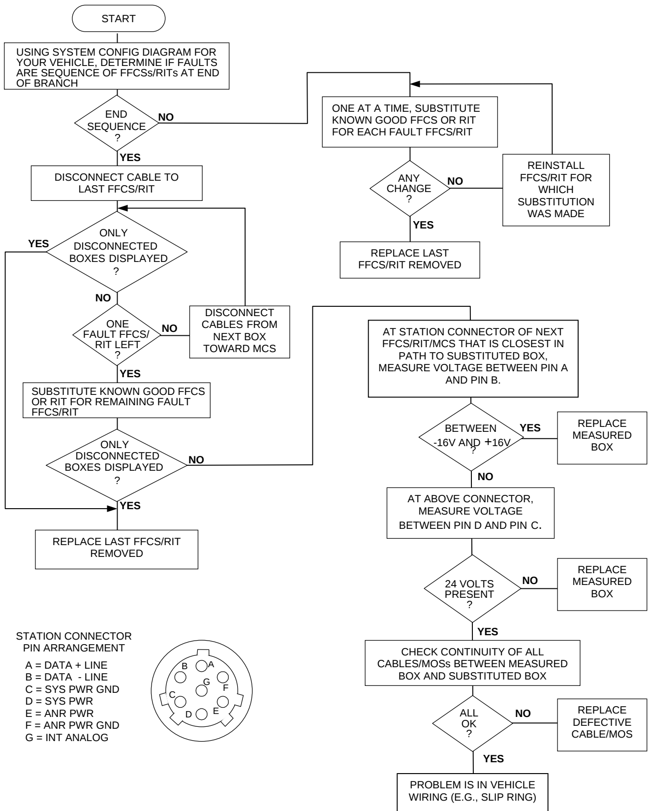
Figure 2-55. Multiple “Xu” Messages for Two-Branch Configuration Flowchart
