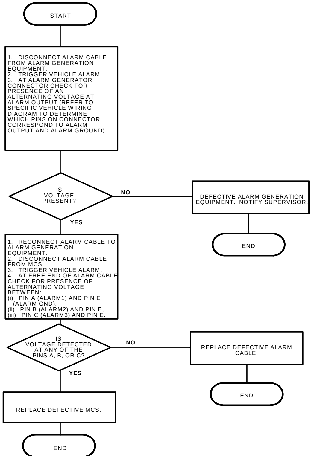
Figure 2-49. Vehicle alarms not heard on intercom Flowchart
