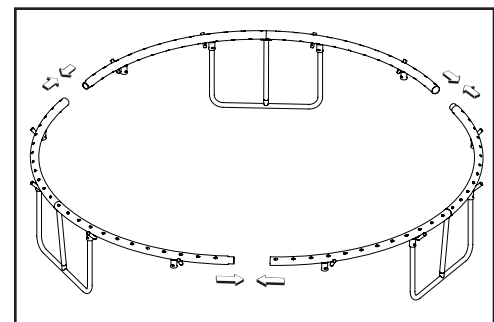
Figure 4: Connecting the frame sections
