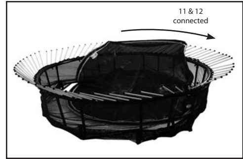
Figure 12-A: Attaching the next (eleventh and twelfth) rods
