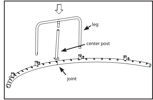
Figure 2-A: Inserting a leg piece and center post
