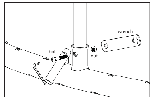
Figure 3: Fastening the legs to the frame
