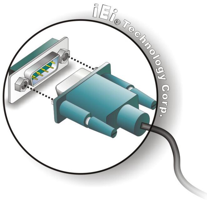
Figure 4-16: DB-9 Serial Port Connector
