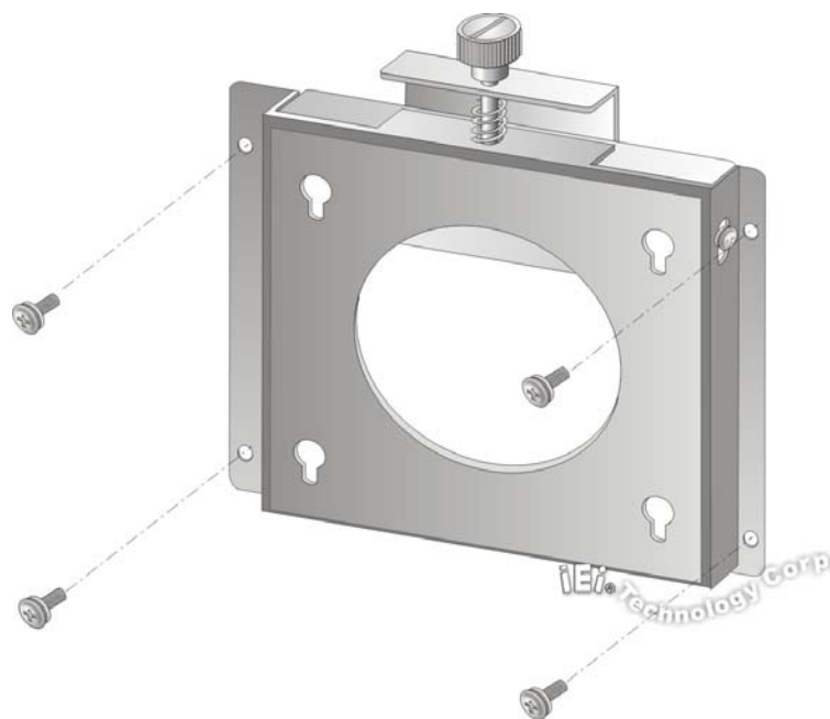
Figure 4-7: Wall-mounting Bracket
