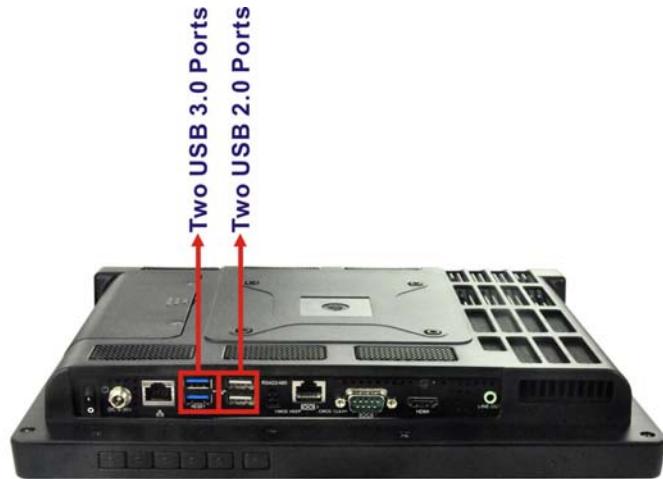
Figure 2-5: External USB Ports
