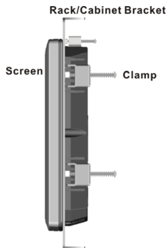
Figure 4-13: Secure the Rack/Cabinet Bracket
