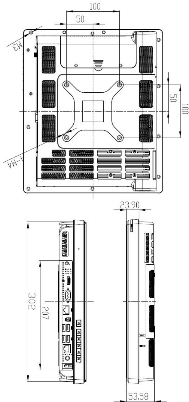
Figure 2-2: AFL2-12A-HM65 Dimensions (mm) cont.
