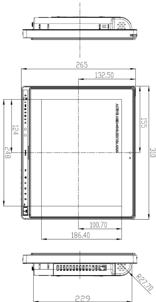
Figure 2-1: AFL2-12A-HM65 Dimensions (mm)
