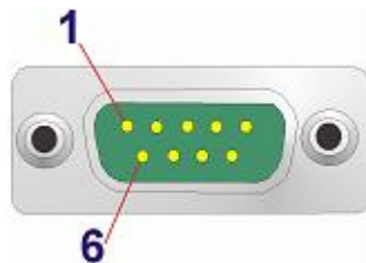
Figure 4-21: DB-9 Connector
