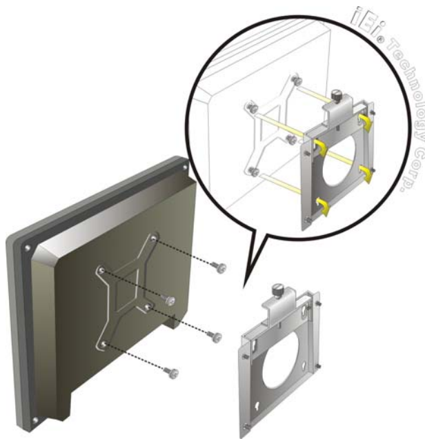
Figure 4-8: Chassis Support Screws
