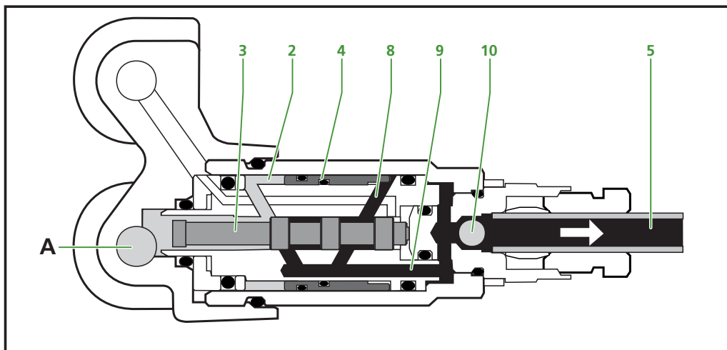
Figure 2.11 Fourth phase
