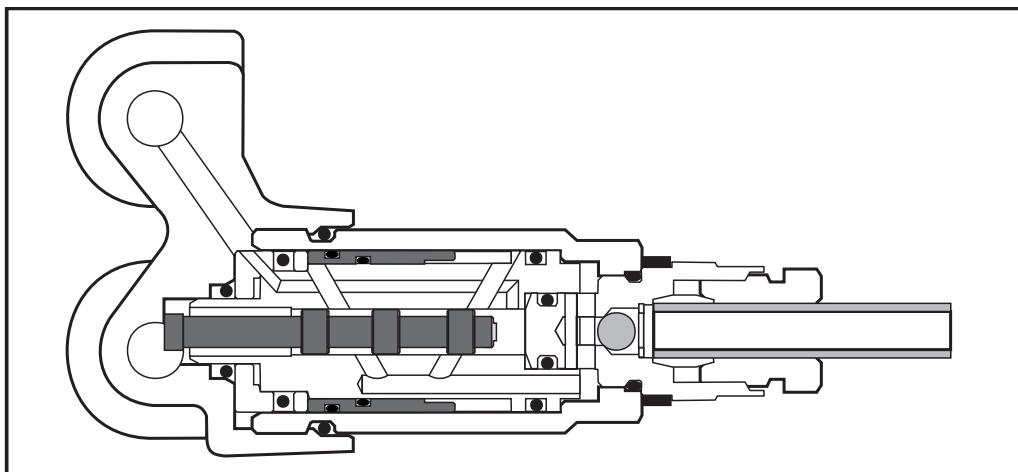
Figure 2.8 First phase
