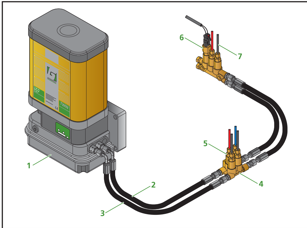
Figure 1.1 System overview
