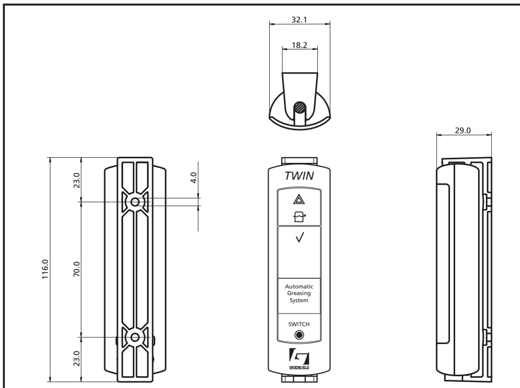
Figure 5.3 Dimensions of the Twin display
