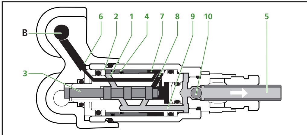
Figure 2.10 Third phase
