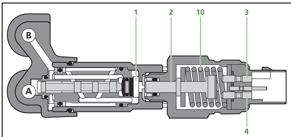
Figure 2.12 First phase
