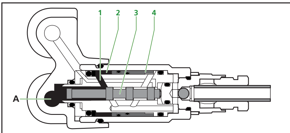
Figure 2.9 Second phase
