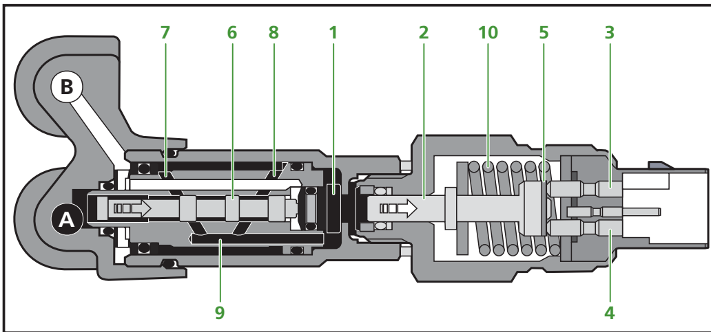
Figure 2.13 Second phase
