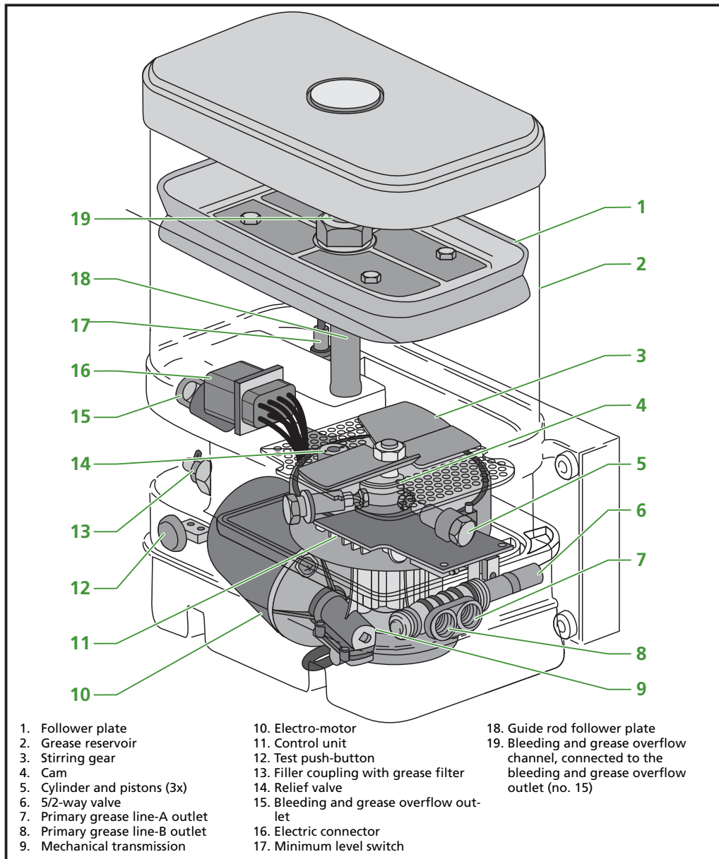
Figure 2.2 Twin pump unit
