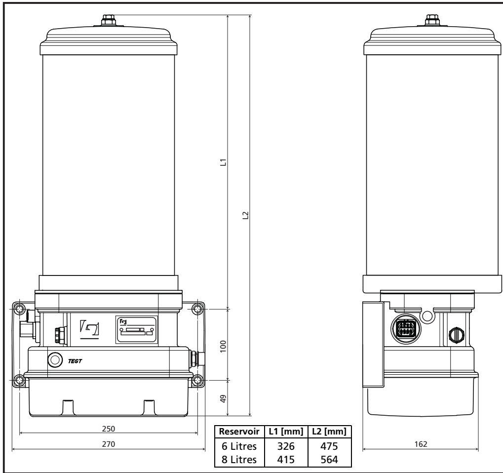
Figure 5.2 Dimensions Twin pump with a 6 or 8 litre reservoir
