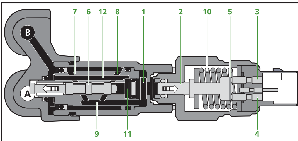
Figure 2.14 Third phase
