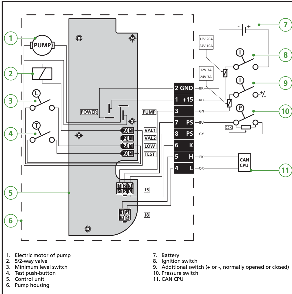
Figure 2.5 Wiring diagram OEM pump with CANbus
