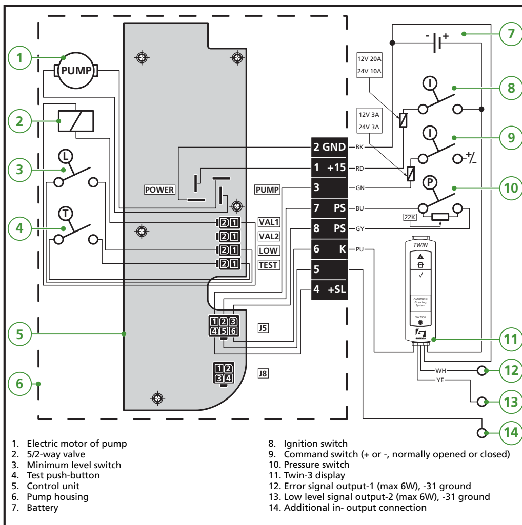
Figure 2.4 Wiring diagram with command switch and Twin-3 display
