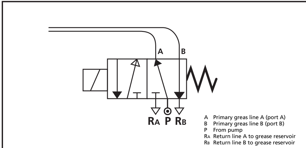
Figure 2.6 5/2-way valve
