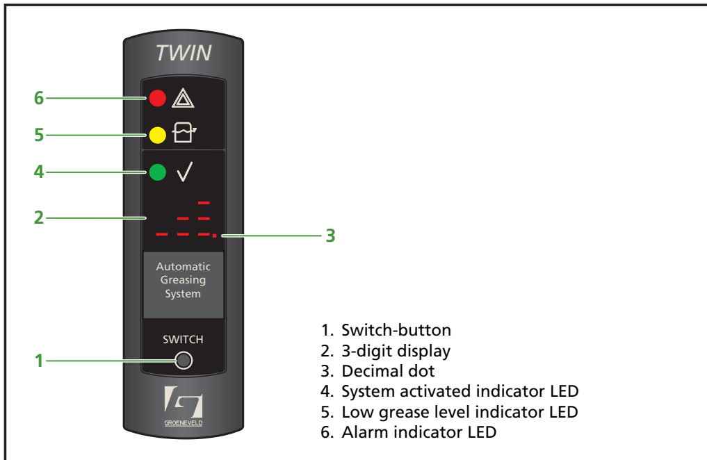
Figure 2.17 Twin-3 display
