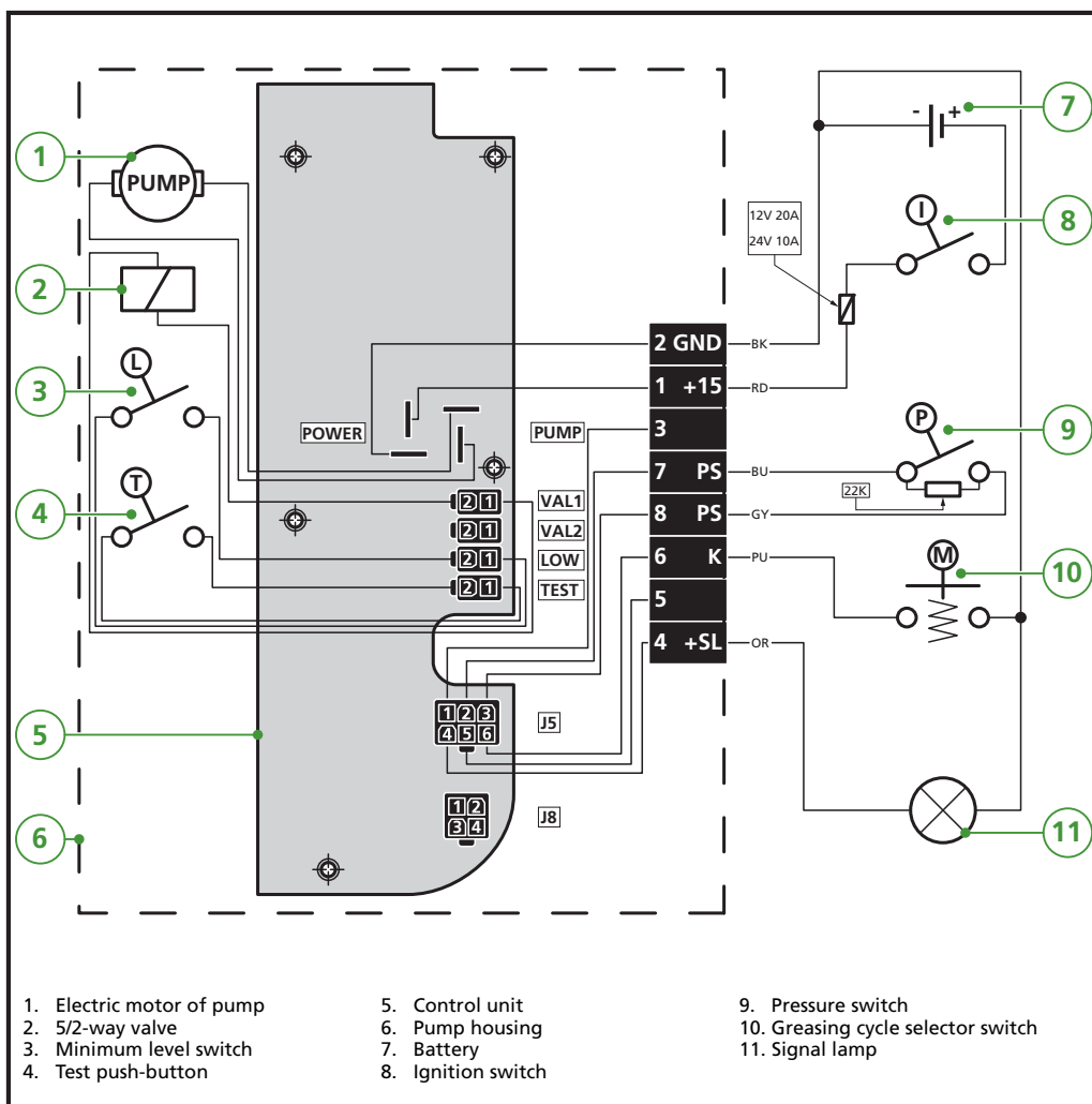
Figure 2.3 Wiring diagram with signal lamp
