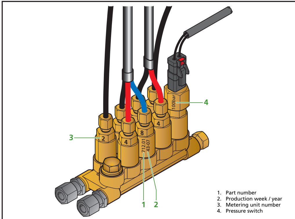
Figure 2.7 Distribution block with metering units
