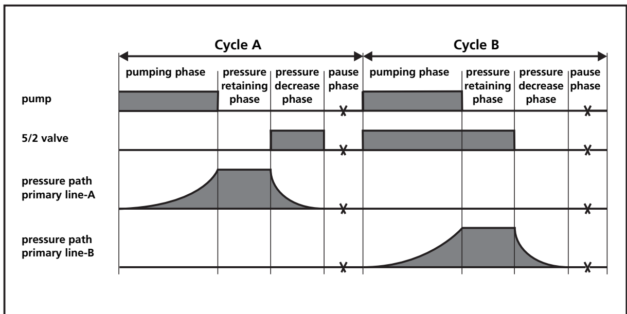
Figure 2.1 Overview of the various phases of the greasing cycle
