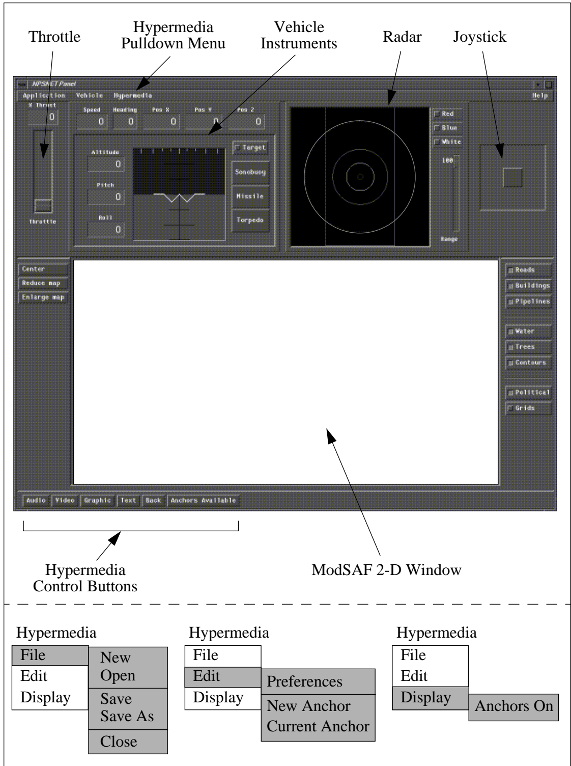
Figure 8: NPSNET Interface Panel and Hypermedia Menus
