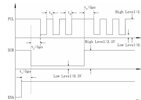
Figure 11: Sequence chart of control signals
