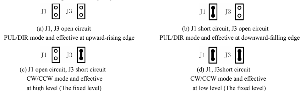
Figure 2: J1 and J3 jumpers
