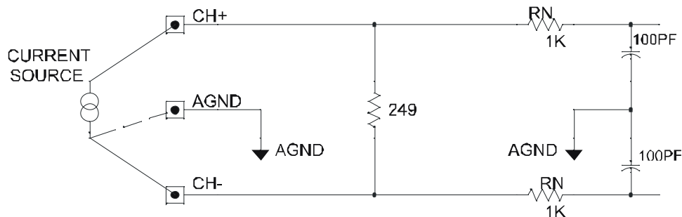
Figure 5-3: Current Input Configuration
