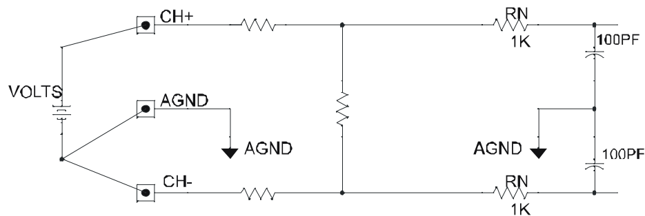
Figure 5-2: Voltage Input With Attenuator
