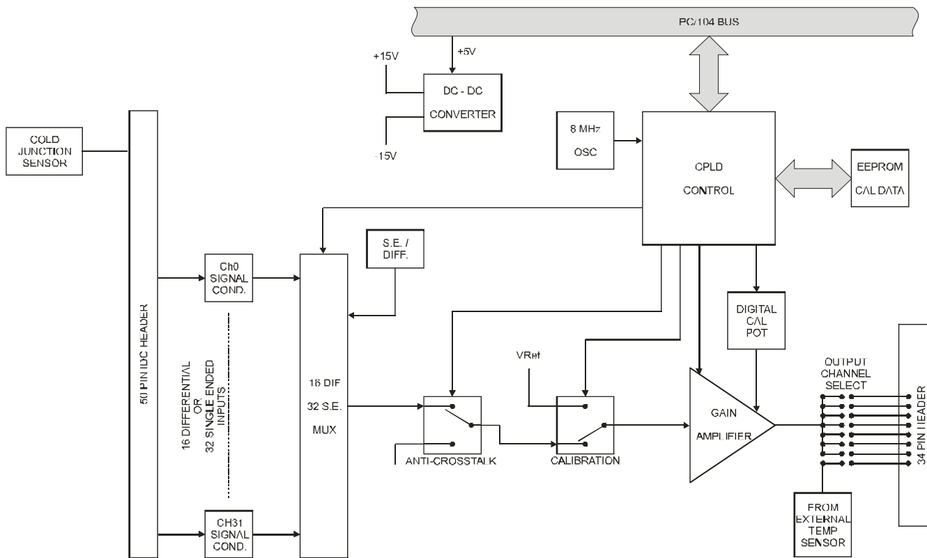
Figure 1-1: Block Diagram
