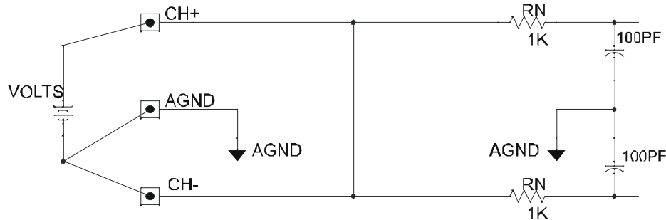
Figure 5-1: Standard Voltage Input Configuration
