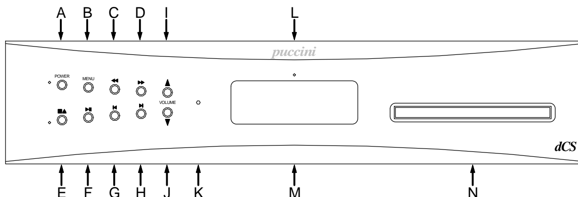
Figure 3 – Front panel
