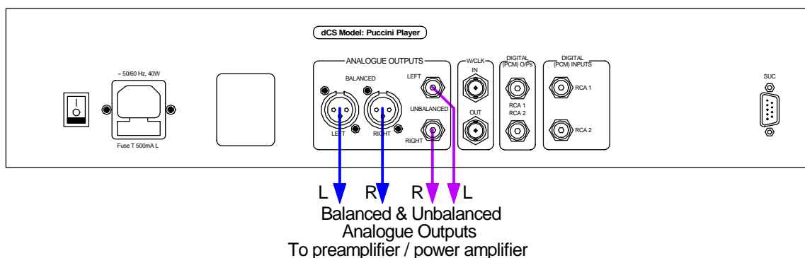
Figure 1 – Basic set-up
