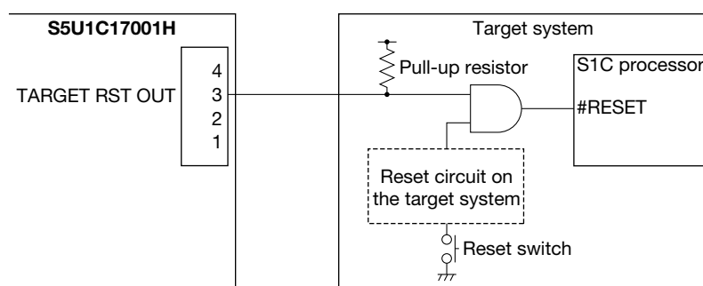
Figure 4.1.2.1 Example of Target Reset Circuit
