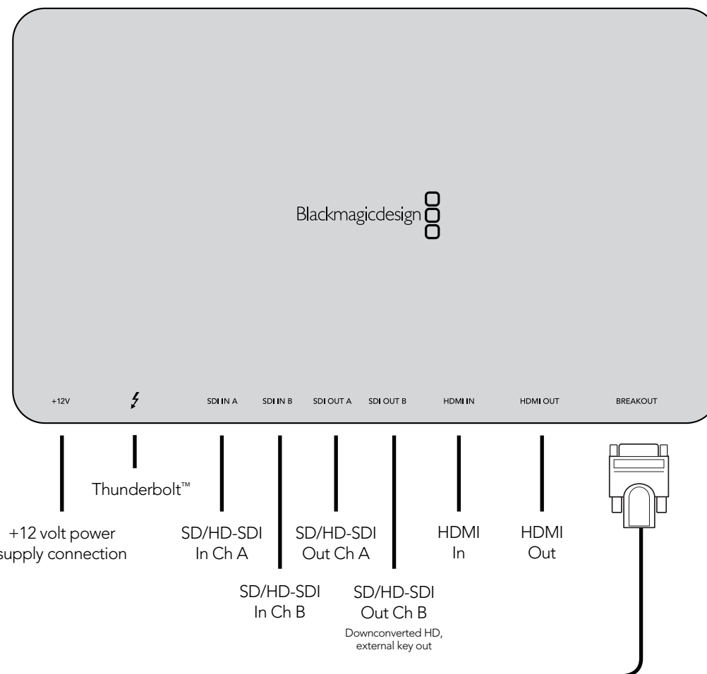
UltraStudio 3D Breakout Cable
