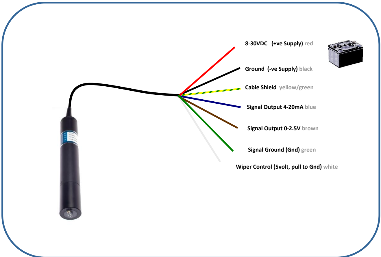
Figure 2 – TS1000 Sensor Connection
