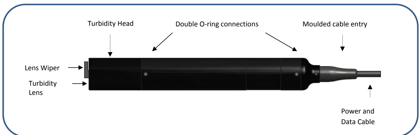
Figure 1 – TS1000 Primary Elements
