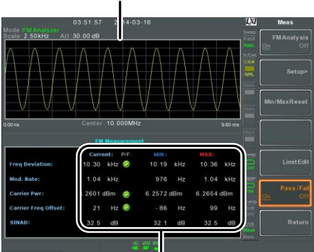
FM modulation measurements
