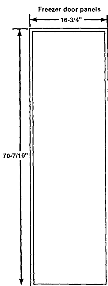
Maximum weight of custom panels is 30 pounds.
