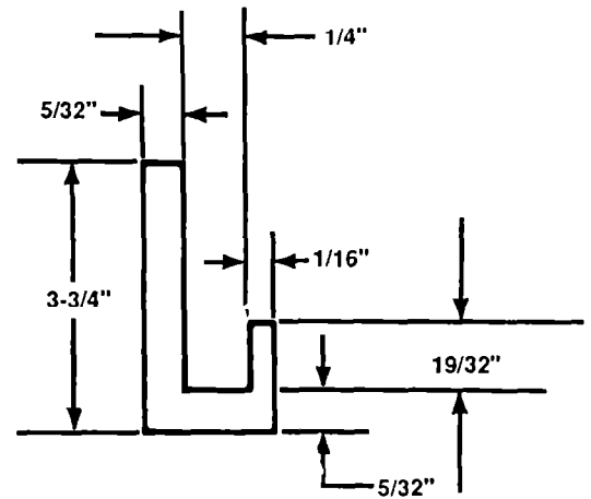
Side trim
