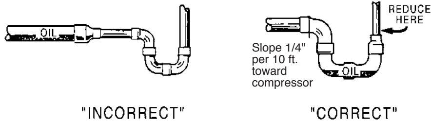
Figure 6. Suction P-Traps.
