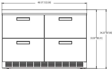
UCD4448N ELEVATION VIEW
