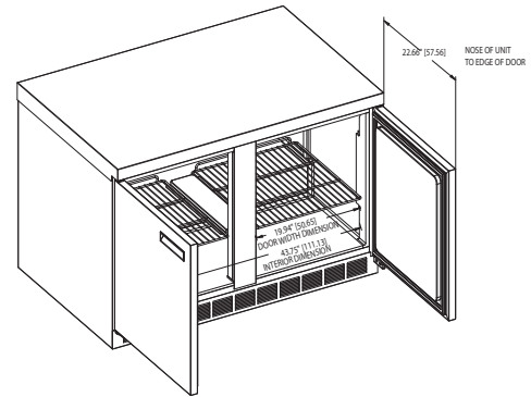
UC4448N ISO VIEW
