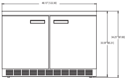
UC4448N ELEVATION VIEW
