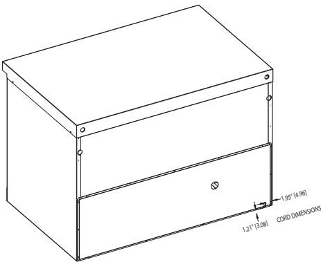
UC4448N & UCD4448N REAR ISO VIEW
