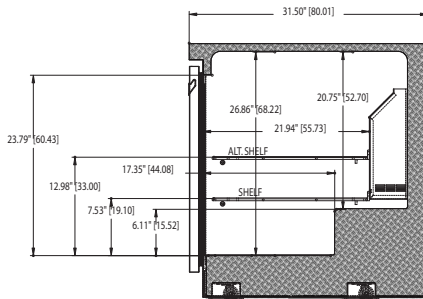
UC4448N RIGHT SIDE VIEW
