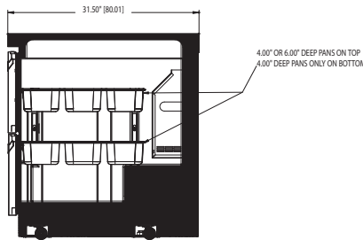
UCD4448N RIGHT SIDE VIEW
