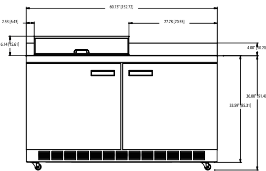
ST4460N-8 ELEVATION VIEW
