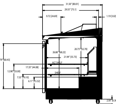
ST4460N-8 RIGHT SIDE VIEW
