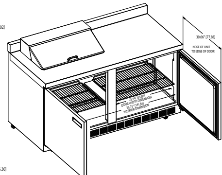
ST4460N-8 ISO VIEW
