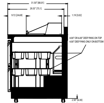
STD4460N-8 RIGHT SIDE VIEW
