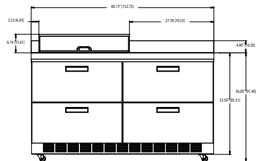
STD4460N-8 ELEVATION VIEW
