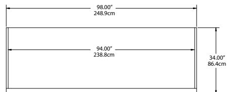
PLAN VIEW SSRRI3-S, SARRI3-S, SMRRI3-S
