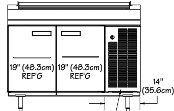
1/4 HP 115V-60C-1PH Elevation View F18RC52
