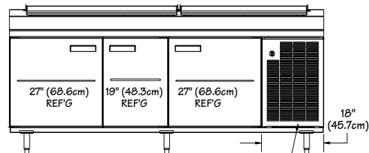
1/2 HP 115V-60C-1PH Elevation View F18RC91
