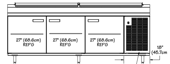
1/2 HP 115V-60C-1PH Elevation View F18RC99
