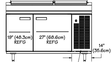
1/3 HP 115V-60C-1PH Elevation View F18RC60
