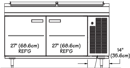
1/3 HP 115V-60C-1PH Elevation View F18RC68
