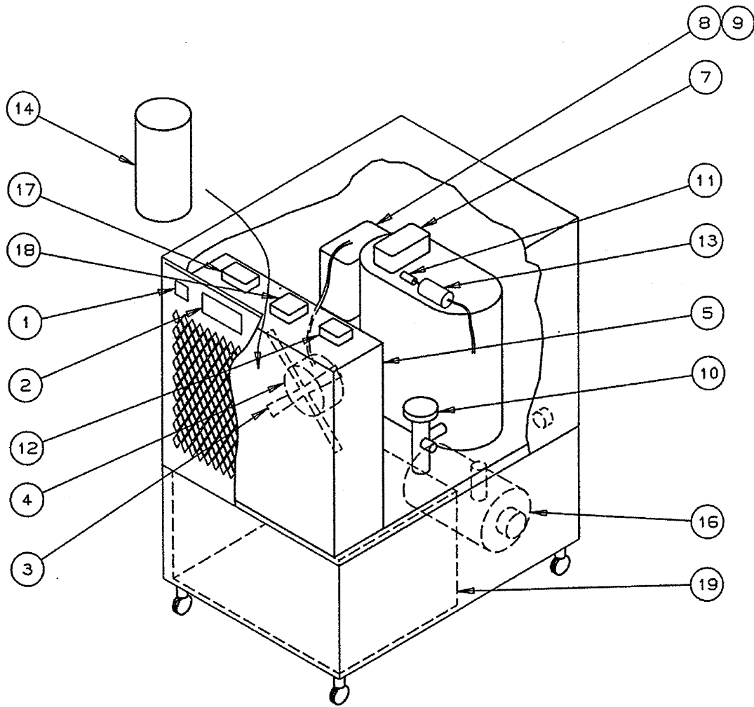
FIGURE 1. CH750, CH751 AND CH951 EXPLODED VIEW
