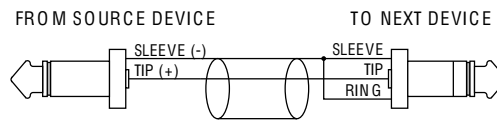
MONO PHONE PLUG TO STEREO PHONE PLUG
