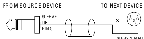
STEREO PHONE PLUG TO MALE XLR-TYPE
