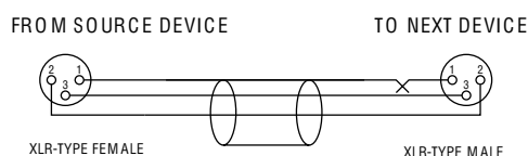
FEMALE XLR-TYPE TO MALE XLR-TYPE
