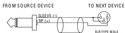
MONO PHONE PLUG TO MALE XLR-TYPE
