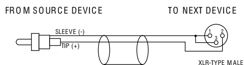
RCA PHONO PLUG TO MALE XLR-TYPE
