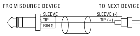
PHONO PLUG TO MALE XLR-TYPE
