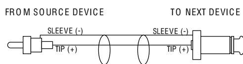
PHONO PLUG TO MONO PHONE PLUG
