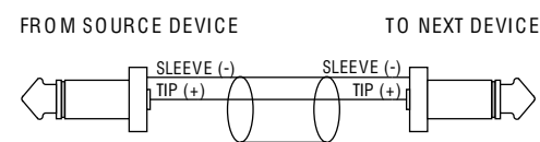
MONO PHONE PLUG TO MONO PHONE PLUG
