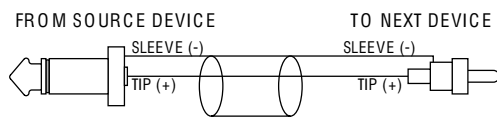
MONO PHONE PLUG TO PHONO PLUG
