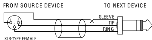
FEMALE XLR-TYPE TO STEREO PHONE PLUG
