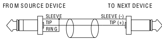
STEREO PHONE PLUG TO MONO PHONE PLUG
