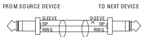
STEREO PHONE PLUG TO STEREO PHONE PLUG
