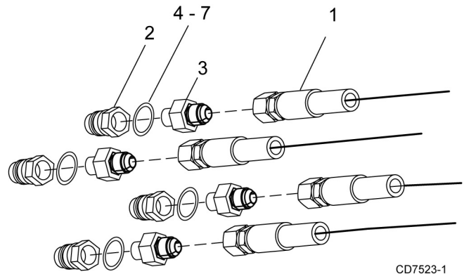
Figure 5. Hose Connections
