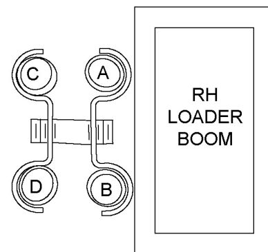
Figure 5. Hose Connections
