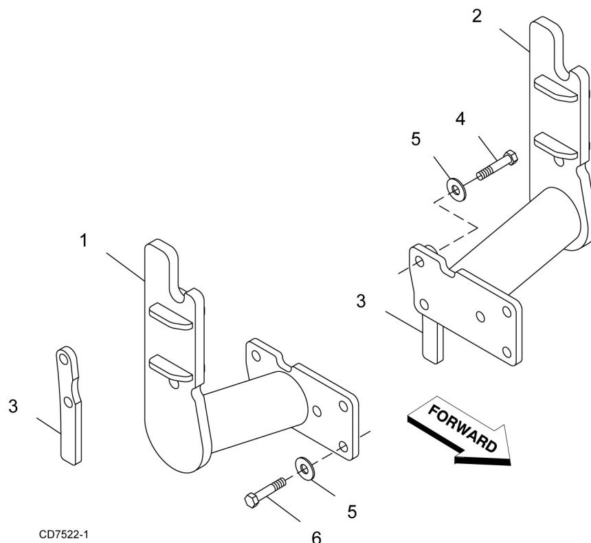
Figure 2. Mount Installation
