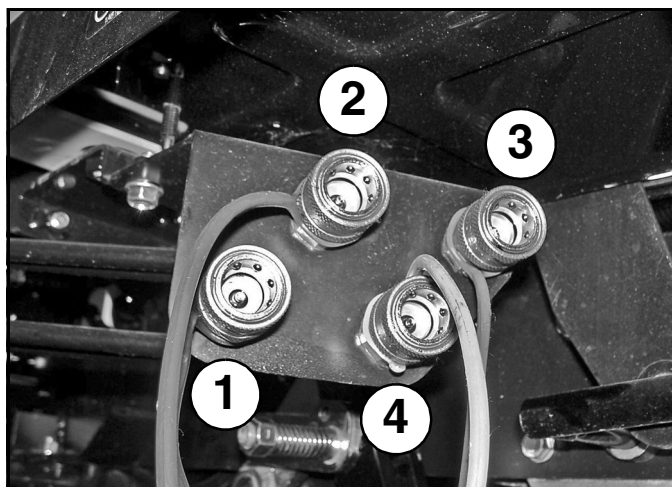
Figure 7. Tractor Hydraulic Remote Connection
