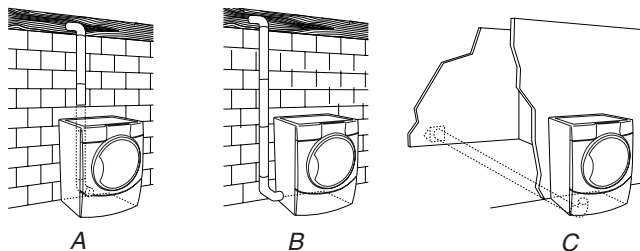
A. Standard rear offset exhaust installation
