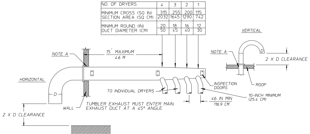
MULTIPLE DRYER VENTING (MLG-78) WITH 10" (25.4 CM) DIAMETER (1200 CFM [34CMM]) EXHAUST CONNECTIONS AT COMMON DUCT
