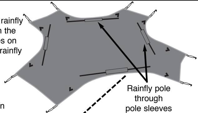
Underside of rainfly attaches to frame poles
