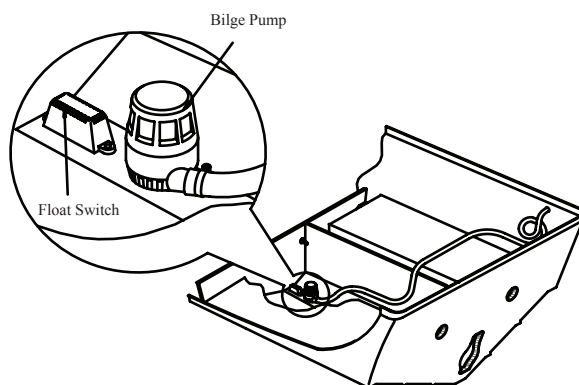
BILGE PUMP AND FLOAT SWITCH (FIG 4.1.2)
