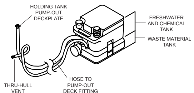
TYPICAL PORTABLE SELF-CONTAINED HEAD WITH DOCKSIDE PUMP-OUT (FIG. 7.4.1)
