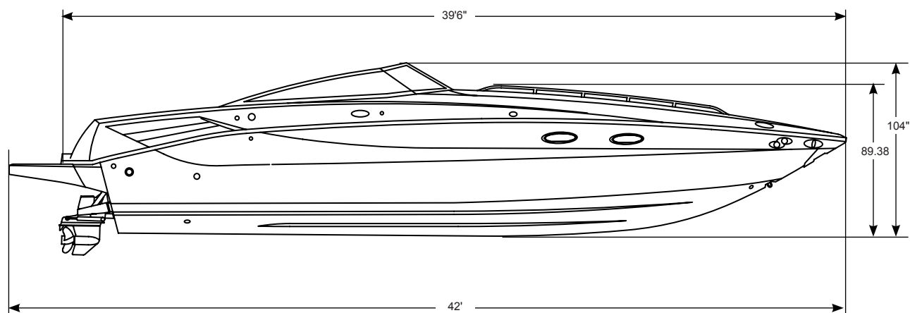
BOAT DIMENSIONS AND CLEARANCES (FIG. 2.2.1)
