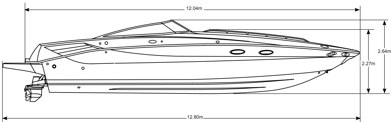
BOAT DIMENSIONS AND CLEARANCES (FIG. 2.3.1)
