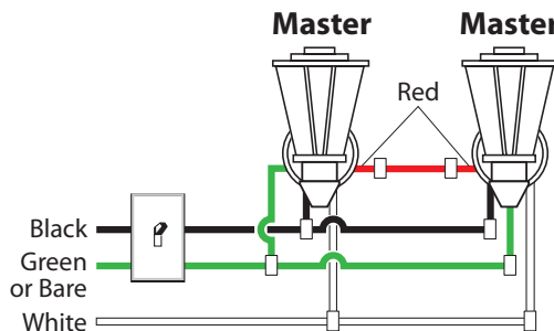
Wiring Diagram 3
