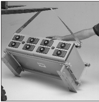
TIP-OVER PROCEDURE Figure 10
