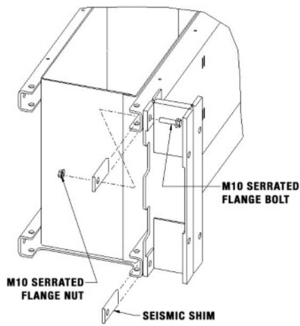
I-BEAM HARDWARE INSTALLATION Figure 7
