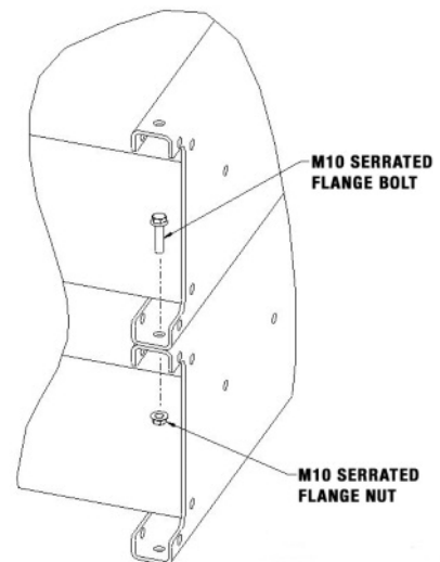
HARDWARE INSTALLATION SEQUENCE Figure 14
