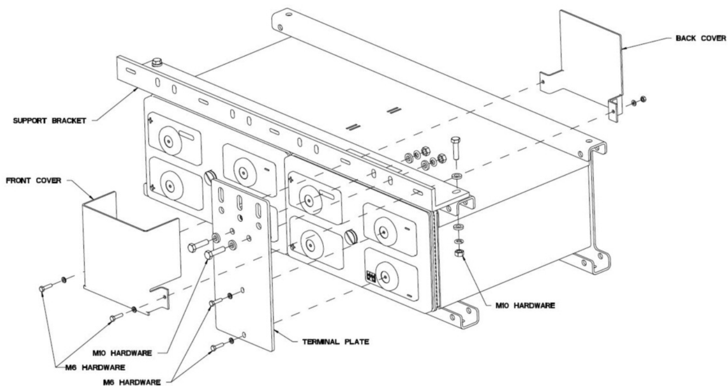
Terminal Plate Kit Materials & Assembly Figure 20
