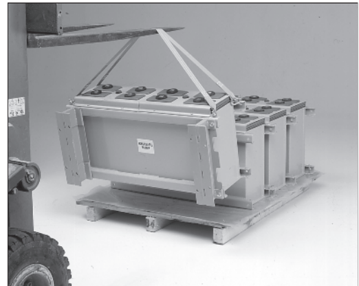
HANDLING MODULE Figure 5
