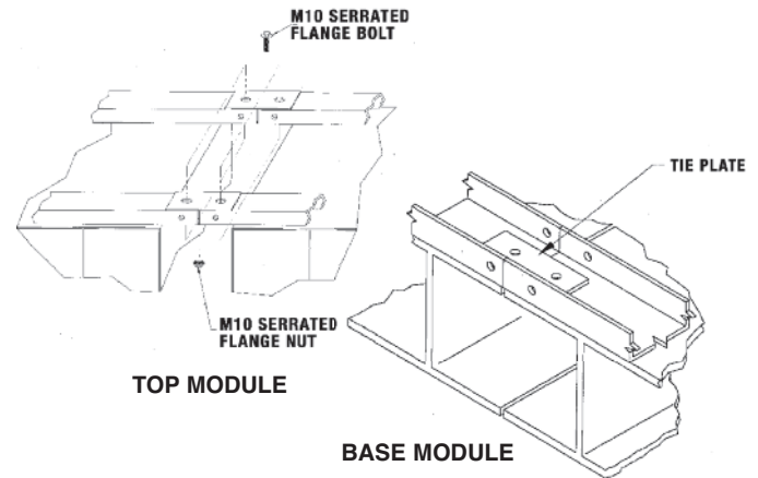
TIE PLATE ASSEMBLIES - HORIZONTAL STACKS Figure 18
