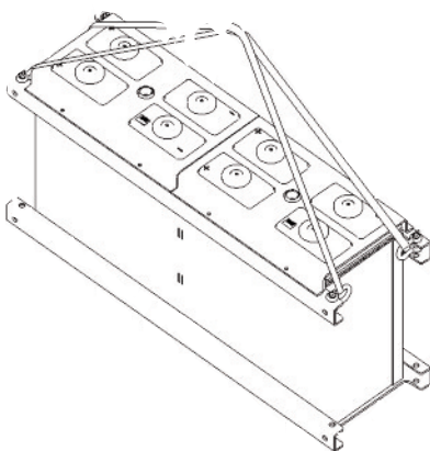
HANDLING - LIFTING STRAP PLACEMENT Figure 4
