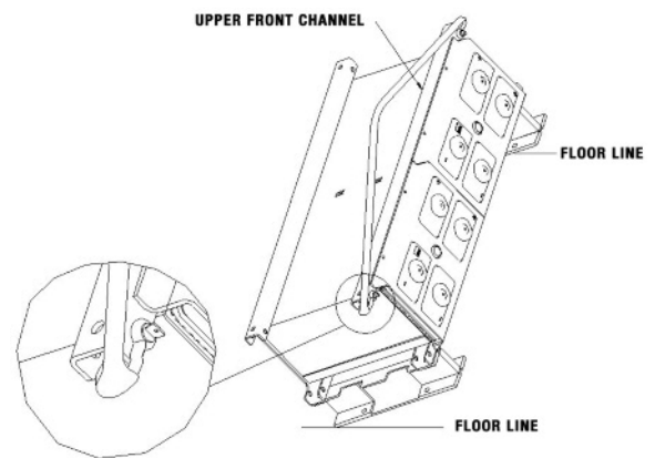
TIP-OVER PROCEDURE - SHACKLE-STRAP USAGE Figure 9
