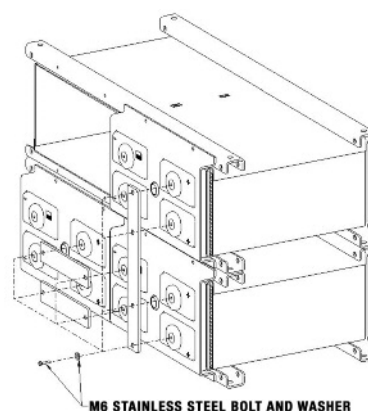
STACK CONNECTIONS Figure 19
