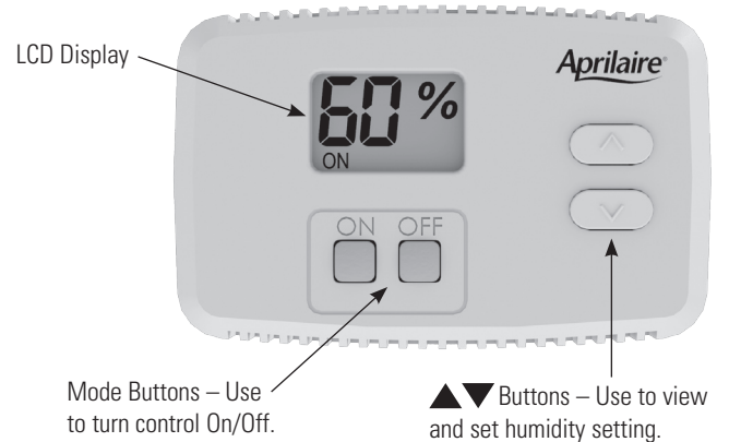
FIGURE 1 – Control Display and User Buttons
