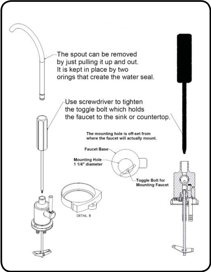
Watts Top Mount Faucet
