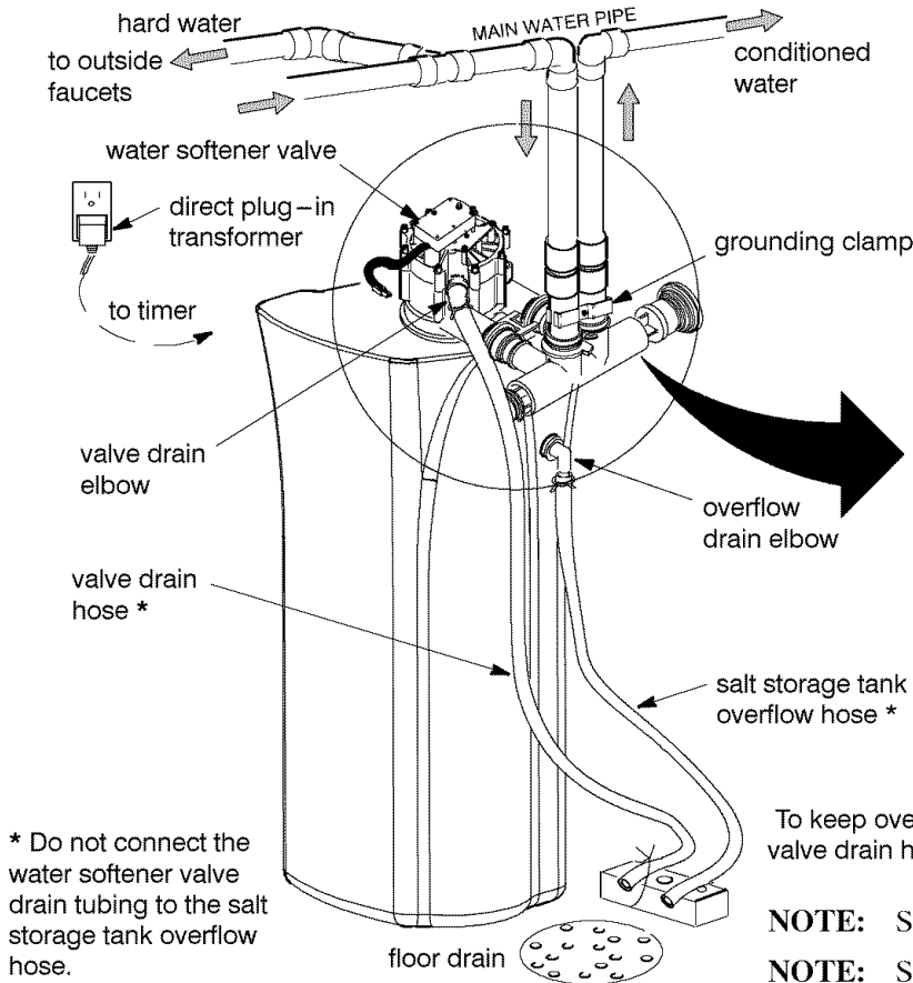
Figure 5 (typical installation)
