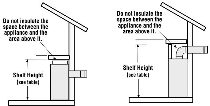
Figure 3 Shelf Above Fireplace With Rear Venting Shelf Above Fireplace With Top Venting
