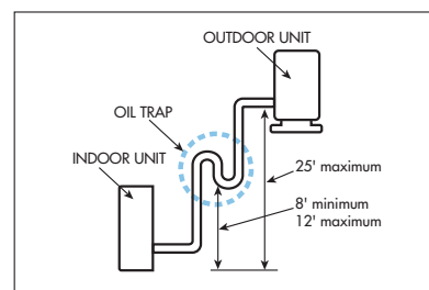
Figure A. Example: 25 ft. maximum elevation. Must install trap inverted.
