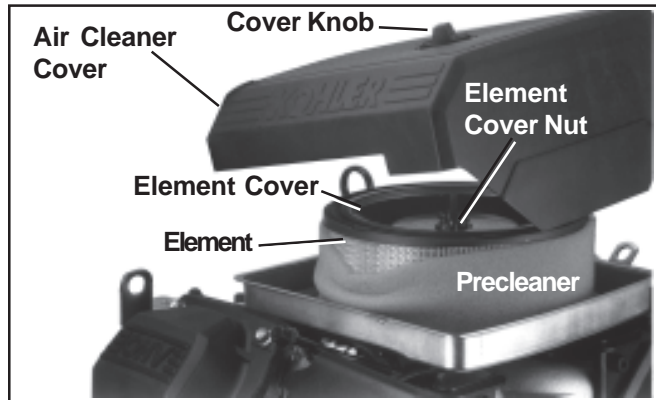
Figure 10. Air Cleaner System Components.
