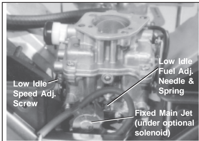
Figure 13. Carburetor (CH18-25).
