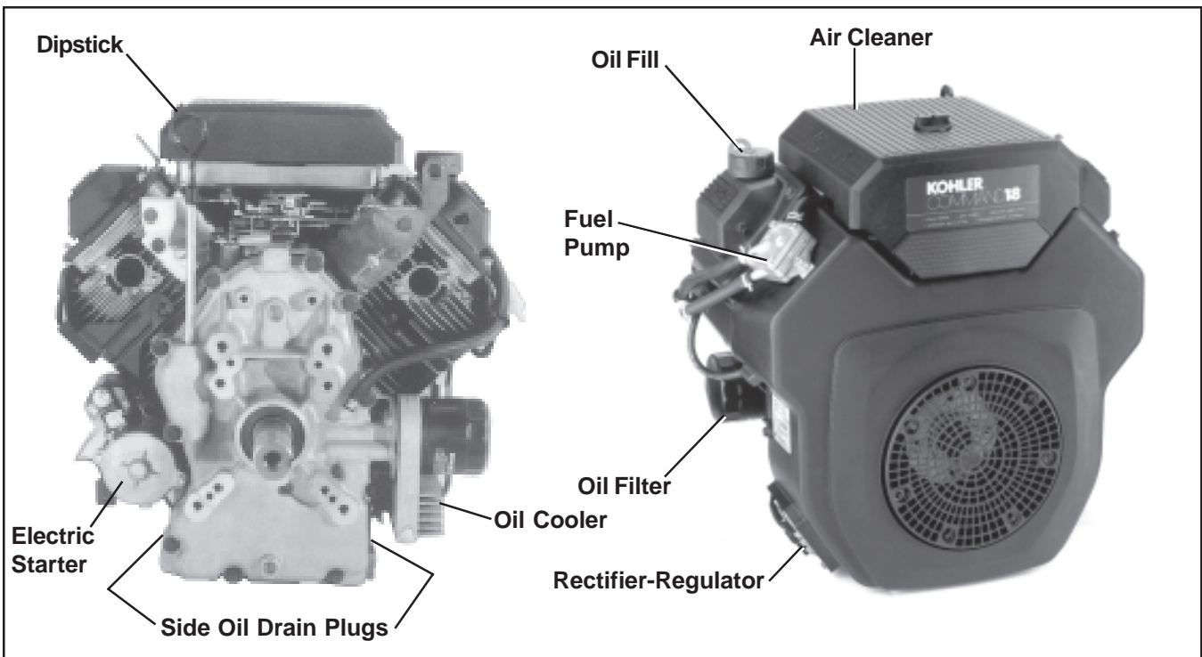
Figure 1. Typical Command Horizontal Shaft Engine (CH18-25).
