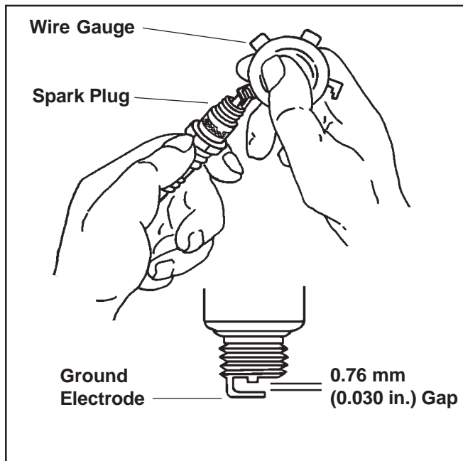
Figure 11. Servicing Spark Plug.
