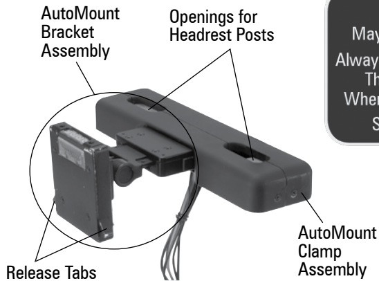
CIOtv AutoMount Assembly
