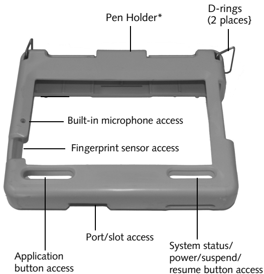
Figure 1. Rugged tablet case - Front
