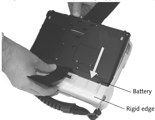
Figure 4. Inserting the system in the case
