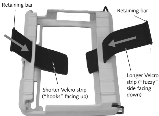
Figure 3. Inserting hand strap halves
