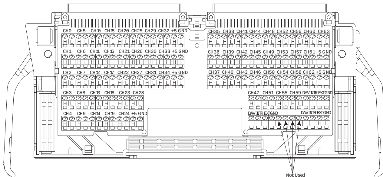
Figure 1-9. HP E1459A Standard Screw-type Terminal Block
