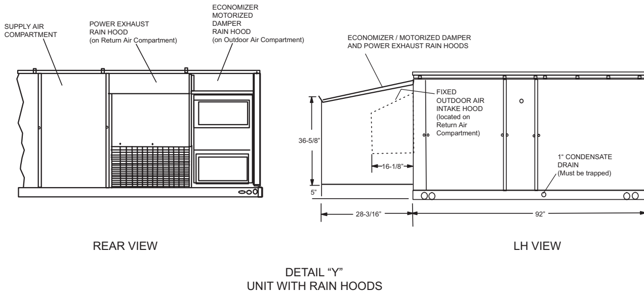
FIGURE 6 - UNIT DIMENSIONS J15, 18, 20 & 25 DJ (RAINHOOD)
