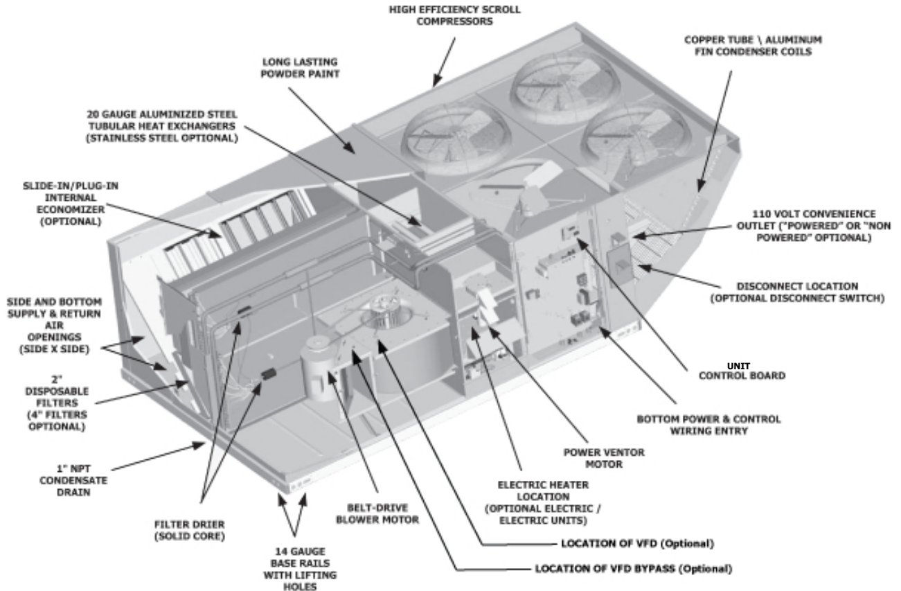
FIGURE 1 - UNIT CUTAWAY
