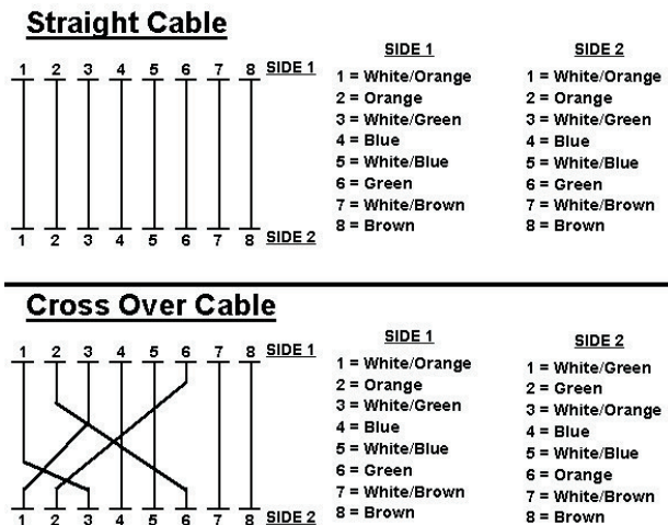
Figure A-1: Straight-Through and Crossover Cable
