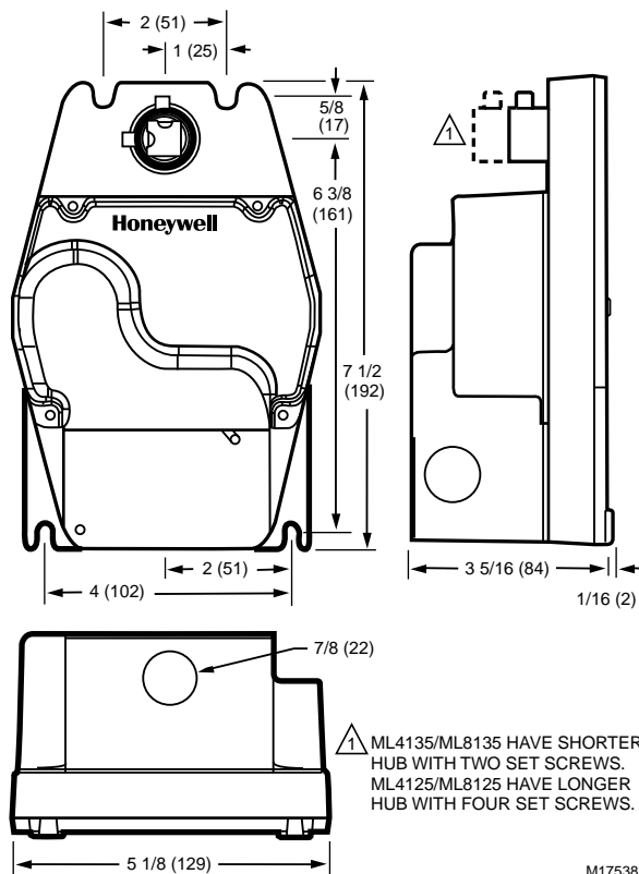
Fig. 1. ML4125/4135, ML8125/8135 dimensiona drawing in in. (mm).
