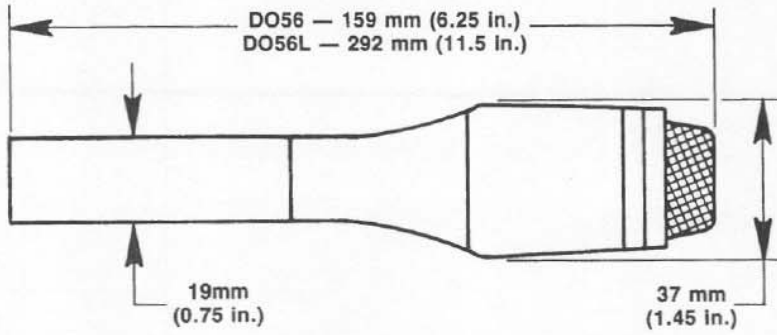
FIGURE 1 — Dimensions
